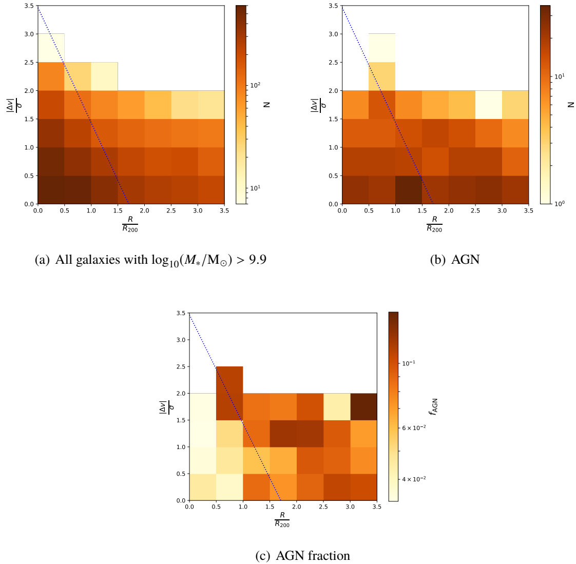
Figure 3.6: Two dimensional histograms showing the projected phase-space distributions of our stacked group of 7498 galaxies. Panel (a) shows the number density of all galaxies, panel (b) shows the number density of AGN, and panel (c) shows the AGN fraction. The blue dotted line shows the modelled infall curve of Oman et al. (2013) . The median absolute error for the AGN fractions in panel (c) is 0.02.
