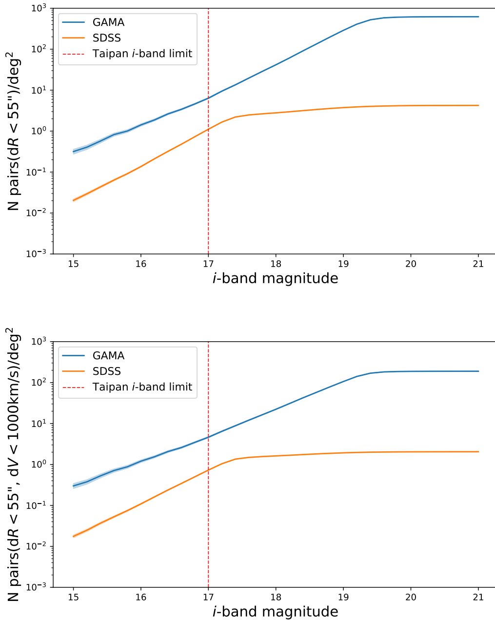
Figure 5.2: The cumulative number density of galaxy pairs separated by less than 55 arc seconds in SDSS and GAMA as a function of i -band magnitude. The bottom panel also requires a velocity separation of no more than 1\,000 \text{ km s}^{-1} , increasing the likelihood that they are indeed bound galaxy pairs and not a chance alignment (Robotham et al., 2014). The blue line represents GAMA, the orange line SDSS, and the red dashed line is the Taipan target selection criteria, i = 17 . The errors shown are Poissonian and of the order of the line thickness at fainter magnitudes.
