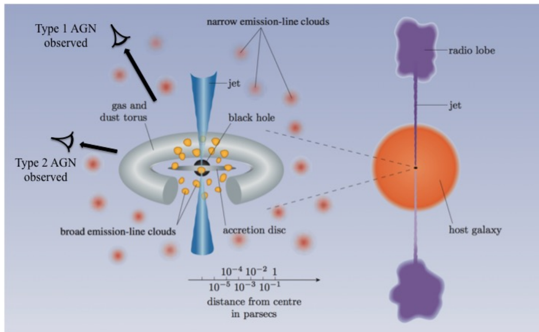
Figure 1.13: Diagram showing a ‘toy model’ of AGN unification. The left hand side shows a close up of the central engine, indicating the relative positions of the black hole, accretion disk, broad- and narrow-line regions, jets (for RLAGN), and the relative orientations of observers for type 1 and 2 AGN. The right hand side shows the relative positions of jets and radio-lobes in the case of RLAGN. Adapted from Serjeant (2010) .
