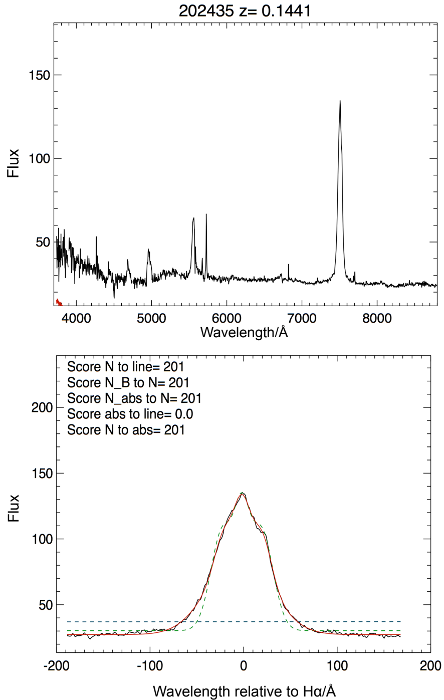
Figure 2.2: Example of Gaussian fit to a broad H\alpha emission line. Top: AAOmega spectrum of the galaxy (GAMA CATAID = 202435). Bottom: fitting of the 6398-6710 \text{\AA} region containing H\alpha and the two [N\text{II}] lines. The score of 201 involving the most complex model ‘N_B to N’ of 201 indicates that this is this is the preferred fit (see Chapter 2.3.3).
