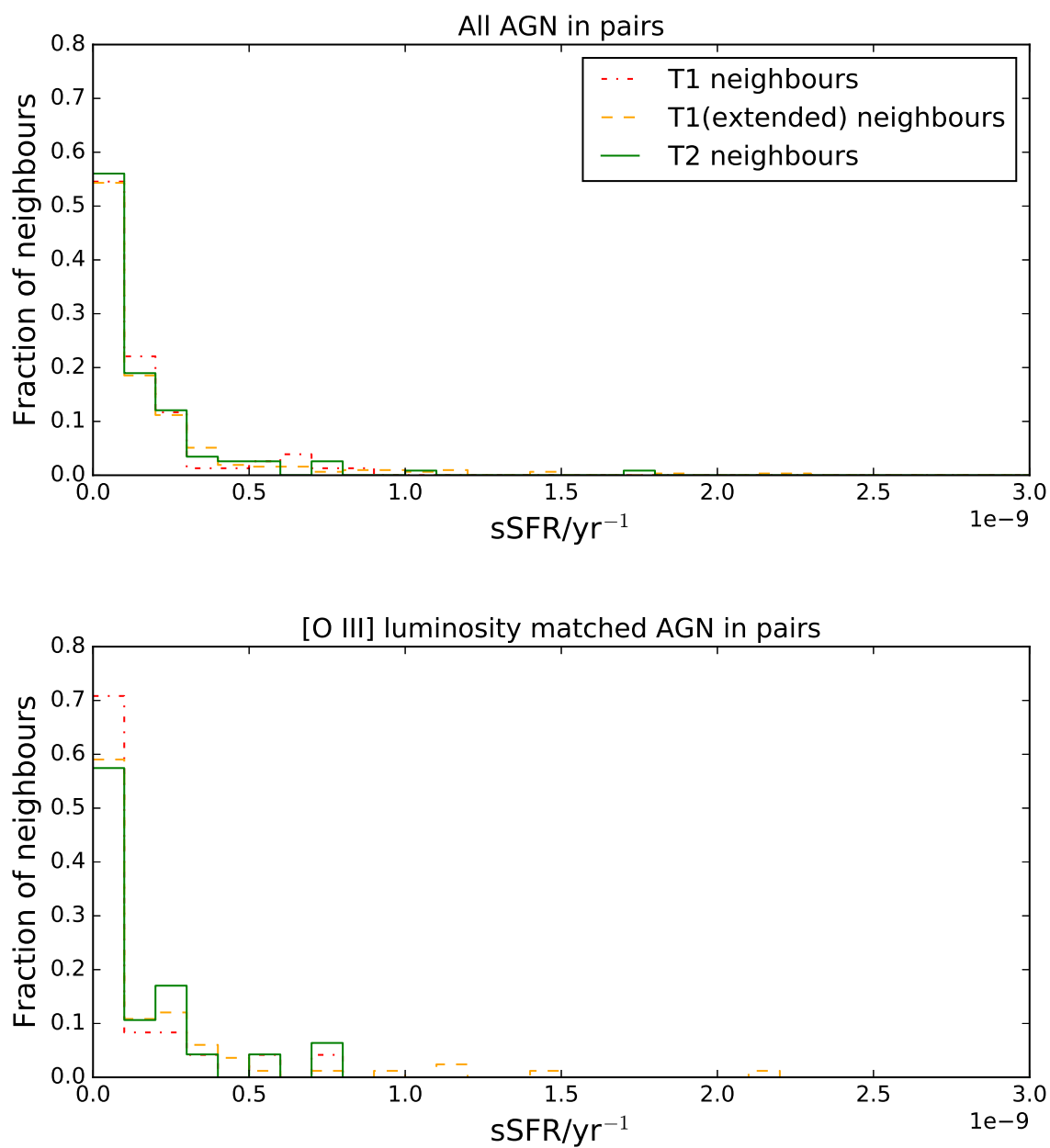
Figure 2.13: Distribution of specific star formation rates for neighbouring galaxies of AGN in pairs which are not themselves AGN hosts and for which reliable emission line data is available. Upper panel: all our AGN in pairs, lower panel: only AGN with 41.5 < \log_{10}(L_{[\text{O III}]}) \leq 42.0 in pairs.
