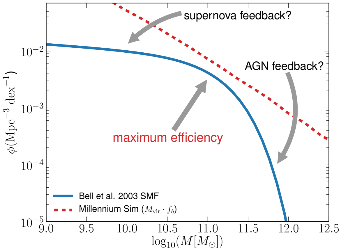
Figure 1.3: A comparison of the stellar mass function based on the observations of Bell et al. (2003, blue curve) to the dark matter halo mass function from the Millennium Simulation (red dashed line, Springel et al., 2005). The different shapes of the functions demonstrated that the efficiency of stellar mass growth is inhibited at both the low and high ends of the stellar mass function, with supernovae and AGN feedback respectively invoked as the causal mechanisms. Originally Fig. 2 in Mutch et al. (2013).
