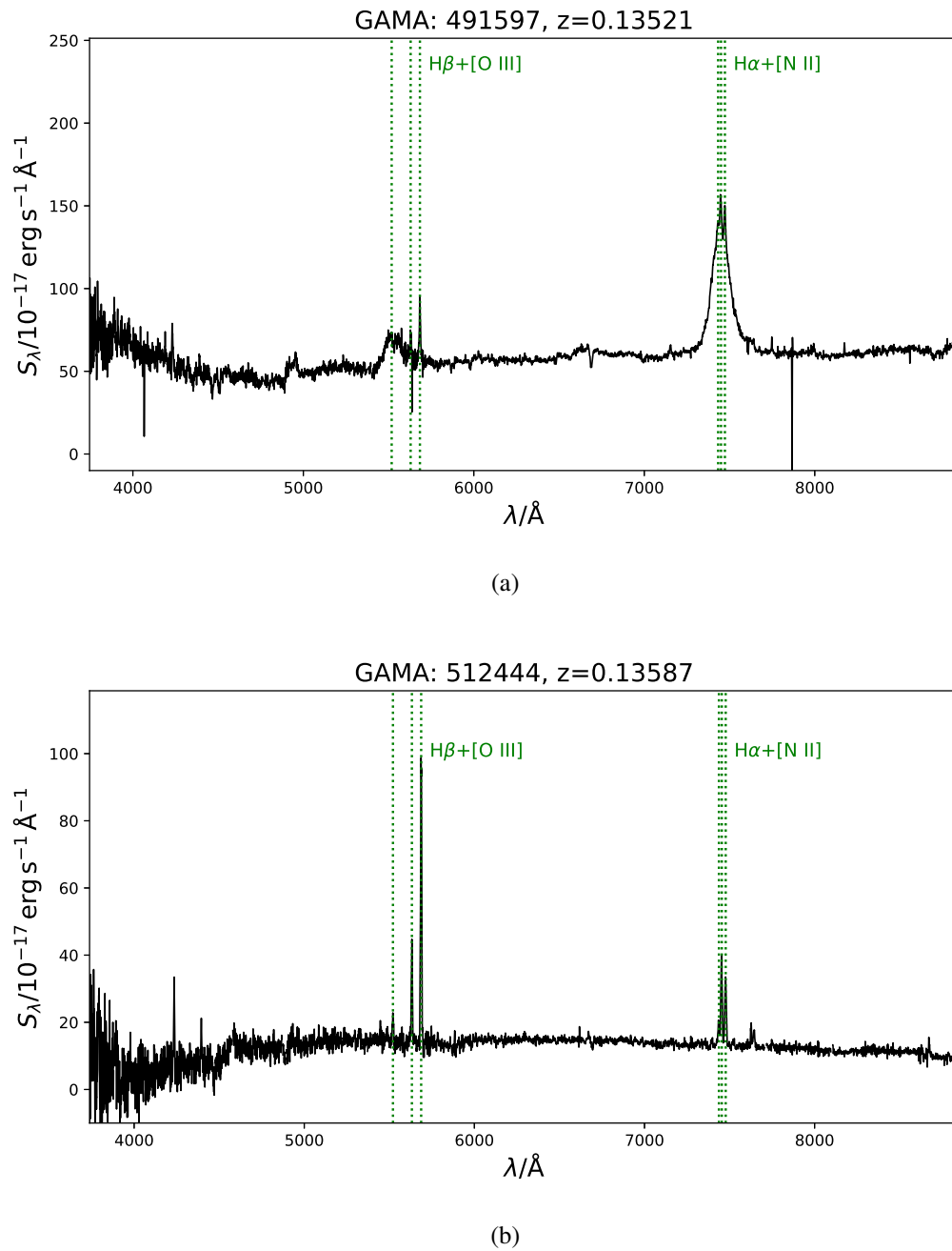
Figure 1.12: Example optical spectra of AGN from the GAMA survey. Panel (a) shows a typical type 1 AGN spectrum. The H\alpha , H\beta , and H\gamma (at just under 5000 \text{ \AA} ) emission lines are substantially broadened. Panel (b) shows a typical type 2 AGN spectrum. No broadening of the Balmer lines is seen, and the only evidence of accretion on to the central SMBH is the presence of the strong [O \text{ III}] and [N \text{ II}] ionisation lines. On both spectra, the GAMA ID and redshift of the galaxy is displayed above the spectrum, and the H\beta+[O \text{ III}] \lambda\lambda 4959 \text{ } 5007 and H\alpha+[N \text{ II}] \lambda\lambda 6548 \text{ } 6583 emission line complexes are highlighted.
