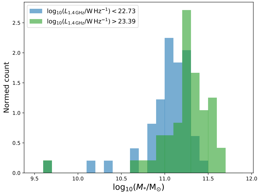
Figure 4.12: The stellar mass distributions of LERGs with \log_{10}(L_{1.4\text{GHz}}/W \text{Hz}^{-1}) > 23.39 (green), and \log_{10}(L_{1.4\text{GHz}}/W \text{Hz}^{-1}) < 22.73 (blue). There is a clear offset in the distributions with a difference in median values of 0.17 dex. That is to say that high power LERGs are \sim 50 per cent more massive than low power LERGs.
