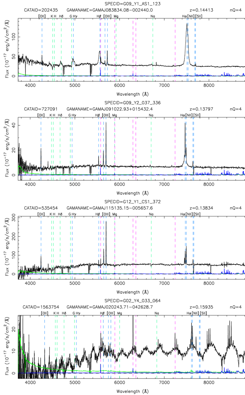
Figure 2.3: From top to bottom: A typical ‘bona fide’ T1 AGN spectrum; a typical ‘intermediate’ type BLAGN spectrum; a typical T2 AGN spectrum; and example AAOmega spectrum affected by time dependent fringing, 19% of our selected broad line spectra were discarded from our data as a result of this. These images are obtained from the GAMA (Driver et al., 2011; Liske et al., 2015) ‘single object viewer’ online tool.
